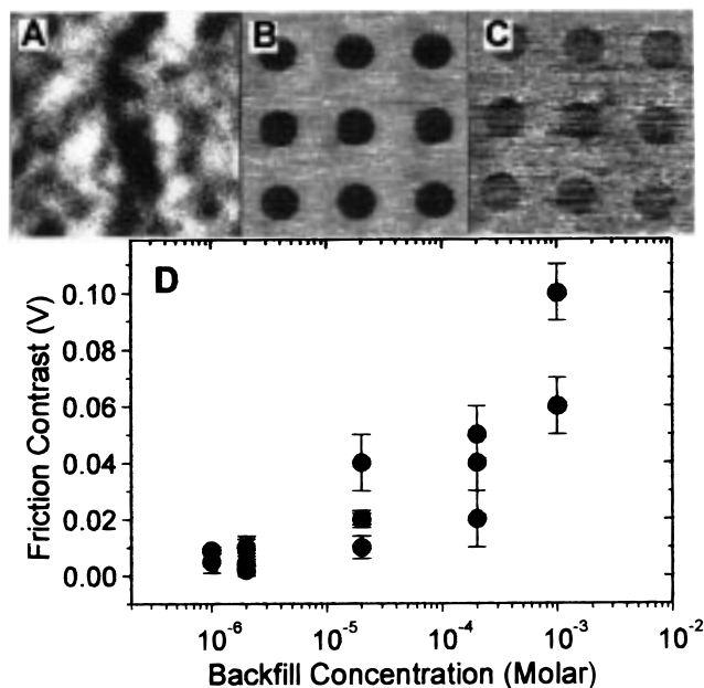
Figure 3. LFM contrast for varied solution backfill concentrations. All three AFM images are for decanethiol monolayers stamped with circles and backfilled with ethanolic solution; all are 60 \mu\text{m} on a side. Part A is the topography of a 1 mM backfilled sample, 3 nm full scale from black to white, and reflects the roughness of the sputtered gold surface. Parts B and C are friction images with a black-to-white full scale of 0.1 V, stamped identically and backfilled with 1 mM and 2 \mu\text{M} solutions, respectively. The lighter the image, the higher the friction, so the stamped regions have lower friction than solution-deposited regions. Part D indicates the average contrast as a function of the backfill solution concentration, as derived from cross-sectional cuts through the images.
